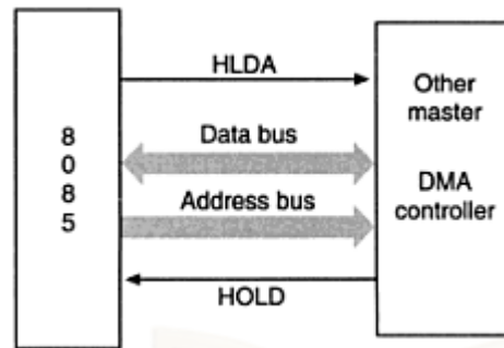
Figure 4-7: HOLD operation
