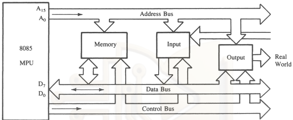
Figure 4-4: 8085 Bus structure
