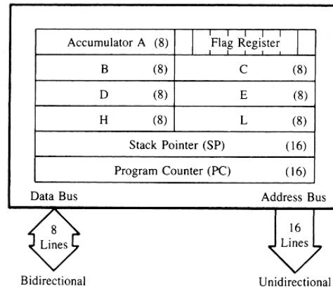
Figure 4-2: Registers of 8085
