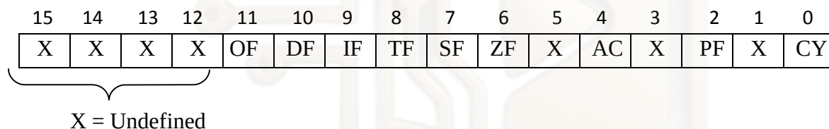
Figure 8-3: Flag Register of 8086
