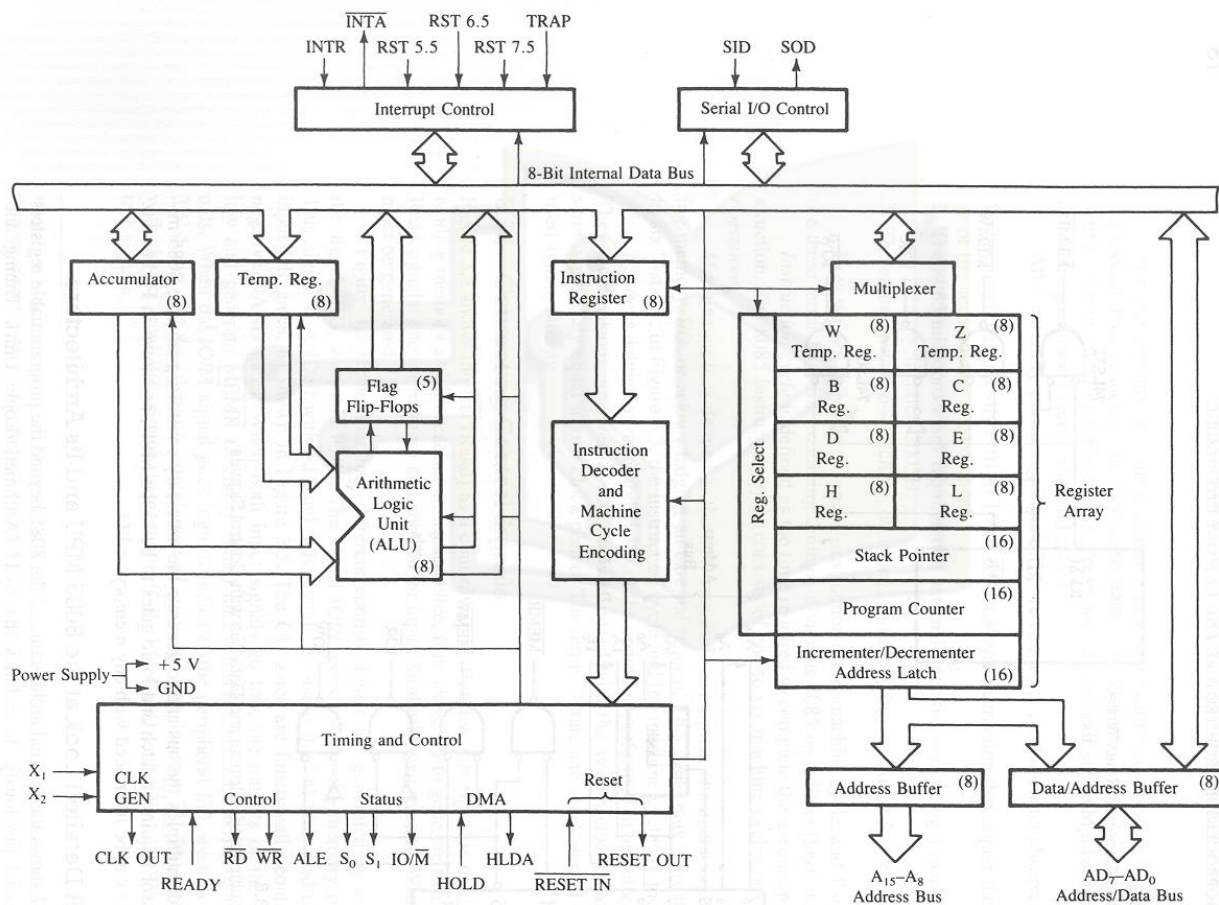
Figure 4-1: Functional block diagram of 8085 microprocessor
